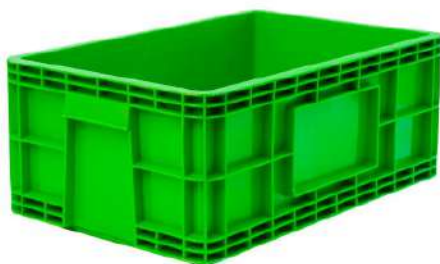
No - 8263 External : 375x580x235 mm. Internal : 340x540x215 mm.
